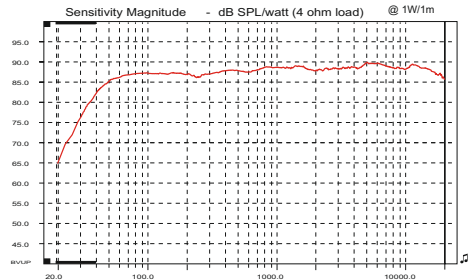
AUDIODESIGN PRO: TRIO LA 6/10 log Frequency - Hz MLSSA: Frequency Domain
